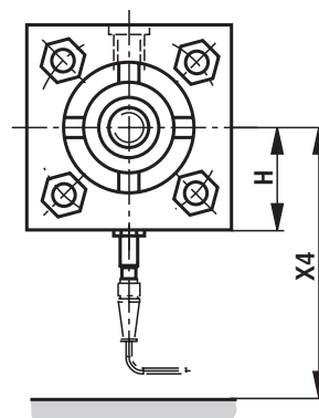
Types of mounting
