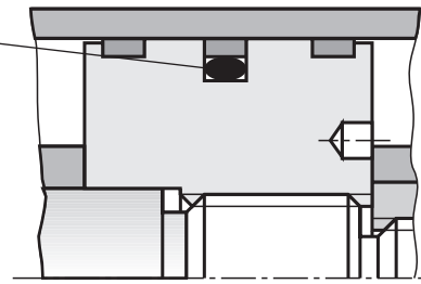
Variant for piston rod Ø 50, 63 and 80 mm
