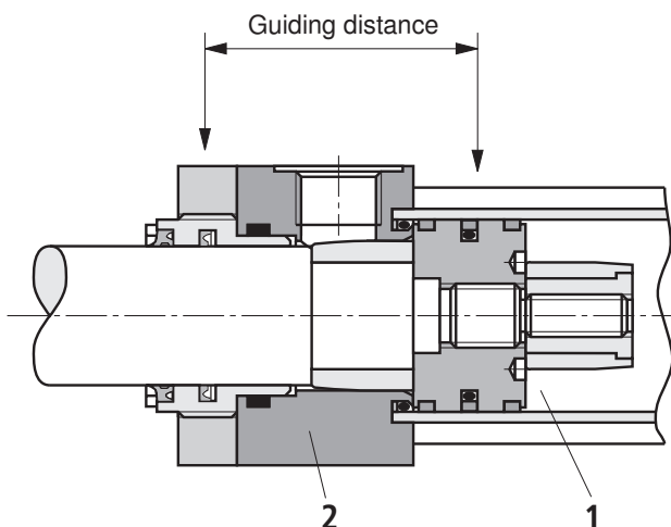
Without stop tube extension
