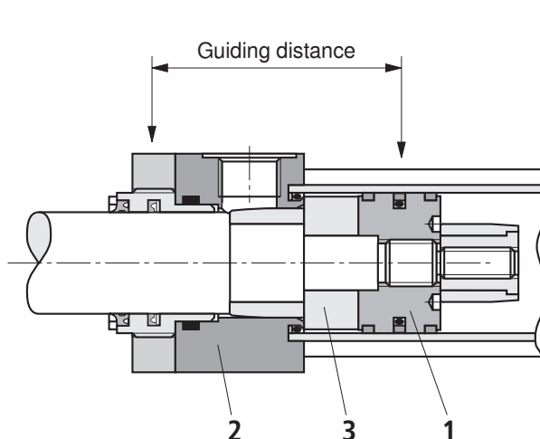
With stop tube extension
