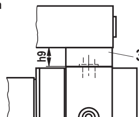
Installation situation with MT4
