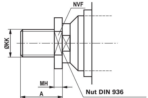
Piston rod end "F"
