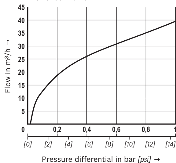
BFSK40-2X / H3V3-M-S-CV with check valve
