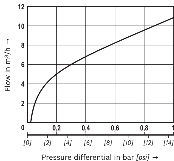
BFSK25-2X / H3V3-M-O-CV with check valve
